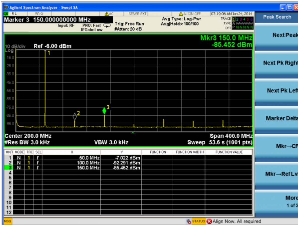
Figure 6. AD9144-EBZ Eval Board output Spectrum
