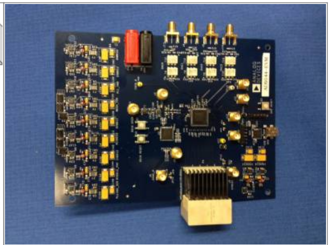
Figure 2. Top view of AD9144-EBZ
